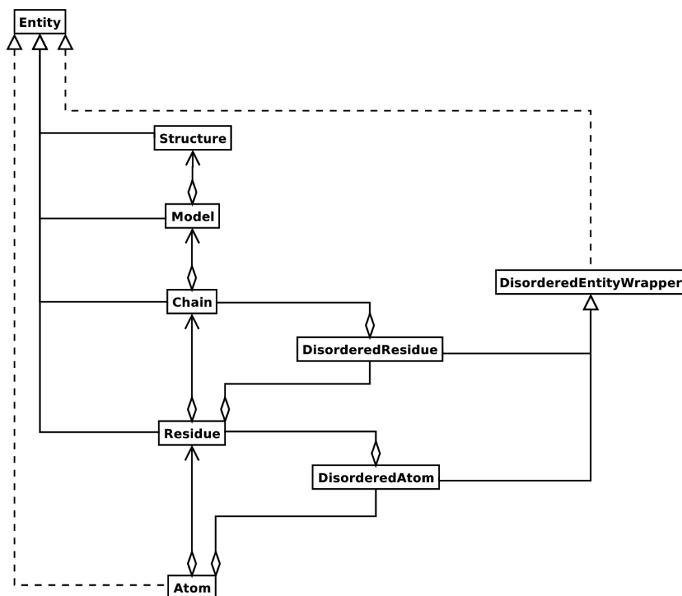
Figure 8.1: UML diagram of the SMCRA data structure used to represent a macromolecular structure.
