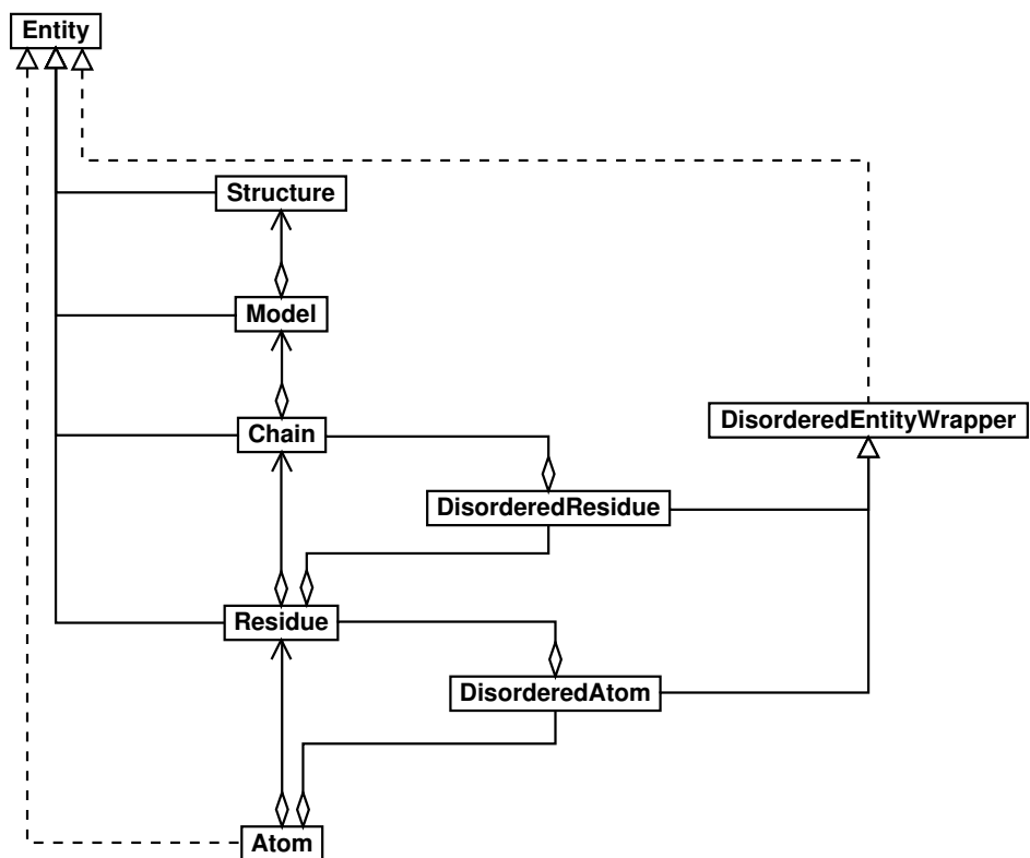
Figure 4.1: UML diagram of the SMCRA data structure used to represent a macromolecular structure.
